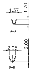
Female terminal
