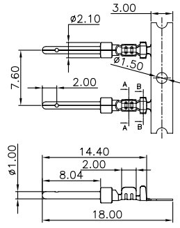
Male terminal
