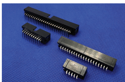
BR5013 CONECTOR BOX HEADER 2,54mm 10 A 64 pinos
