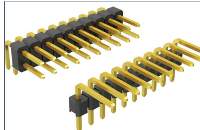
DS1022 BARRA DE PINOS PASSO 2,54mm 90 GRAUS
