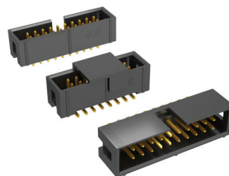
DS1013 CONECTORES BOX HEADER 2,54mm 10 A 64 PINOS
