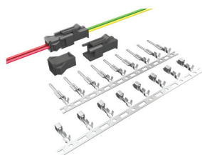
DS1068-02 CONECTOR CABO A CABO PASSO 2,5mm (Equivalente JST-SMP/SMR)
